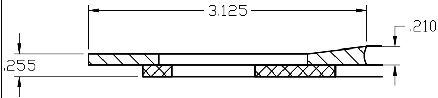
DETAIL A SCALE 3:1
